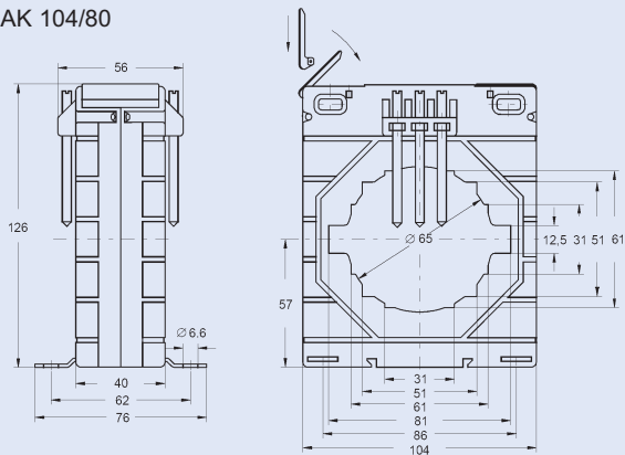
MAK 104/80
